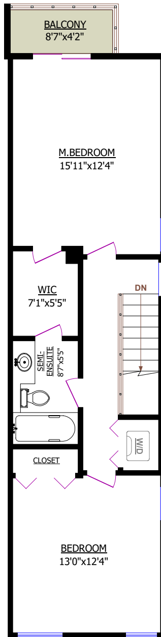
UPPER LEVEL
